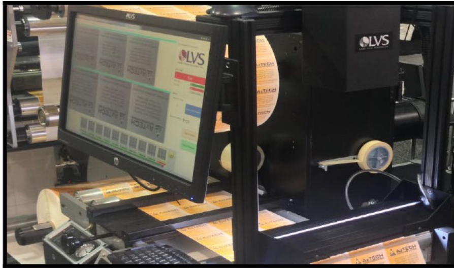
LVS® 7300 Mounted to Aztech's High-Speed Slitter Rewinder Inspector
